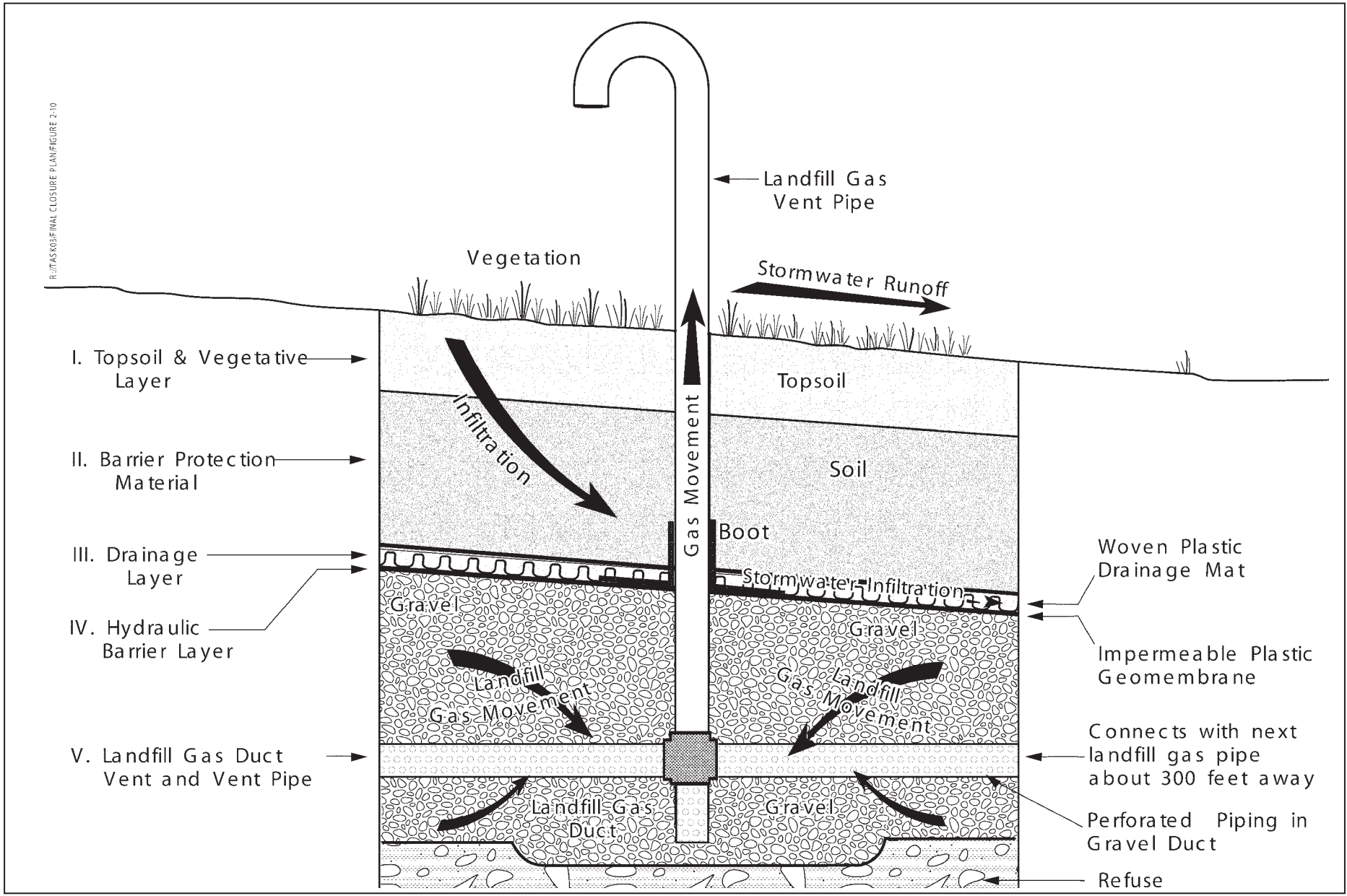
Final Cover and Landfill Gas Venting System: Landfill Sections 2/8 and 3/4 Figure 21-3
